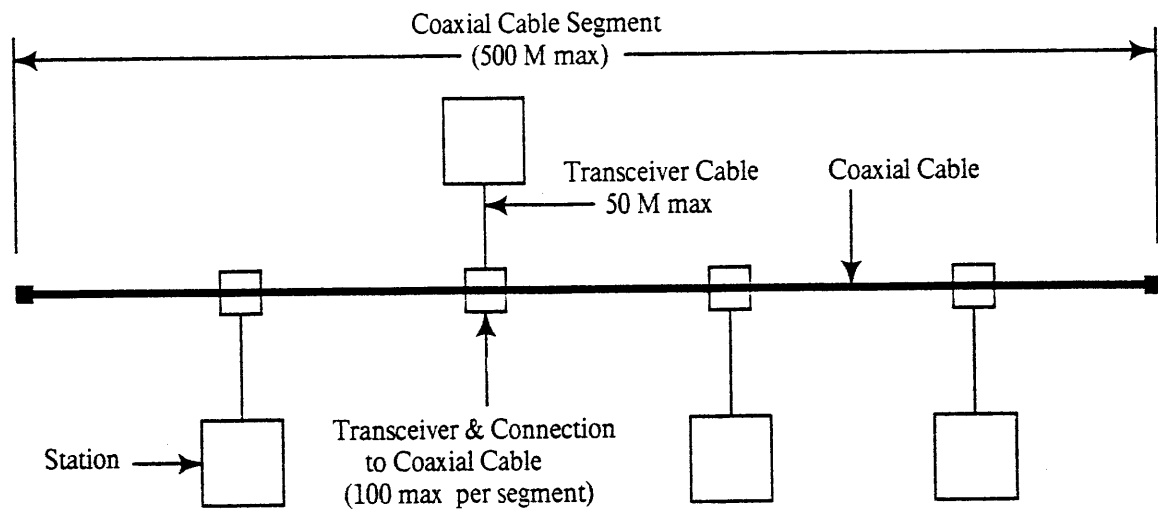
Figure 7-1a: Minimal Configuration
