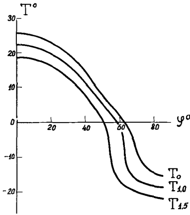
Fig. 4. The dependence of temperature distribution on radiation amount.
