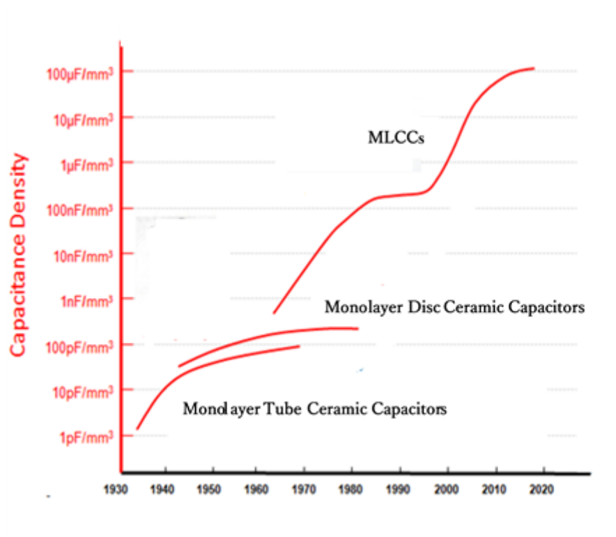
Fig. 1 Changes of capacitance densities of monolayer/multilayer ceramic capacitors
