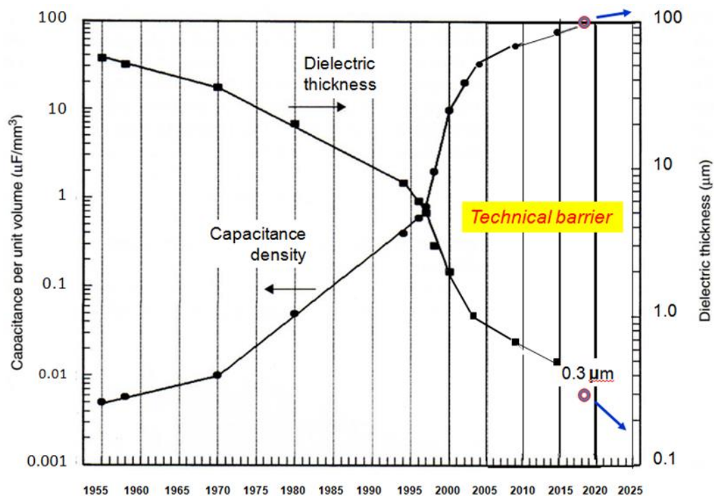
Fig. 2 Changes of capacitance density and dielectric thickness of MLCC
