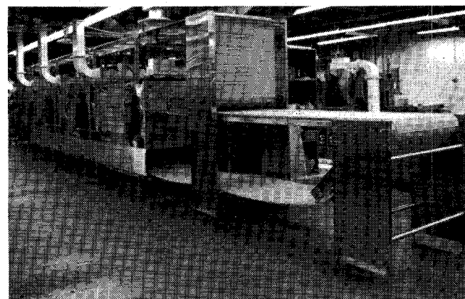
Fig. 24. A 240-kW bacon-cooker conveyorized system which operates at 915 GHz. (Photo courtesy of Raytheon Co., Microwave and Power Division.)
