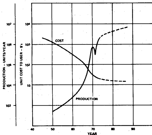
Fig. 17. Production figures and user unit costs of cooker magnetrons past and projected (taken from H. K. Jenny, "Electron tubes—A technology forecast," Technology Trends (75CH1005-8 TFA), IEEE, NY (1975)).
