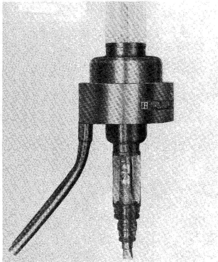
Fig. 7. The Litton magnetron L3858, made for use in early microwave ovens like the Tappan wall models. (Photo courtesy of Gerling Laboratories.)
