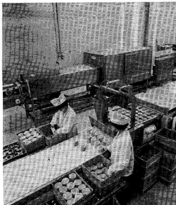
Fig. 22. Meat-tempering tunnel conveyor (Raytheon) which operates at 915 MHz with power levels up to 200 kW. (Photo courtesy of Raytheon Co., Microwave and Power Division.)
