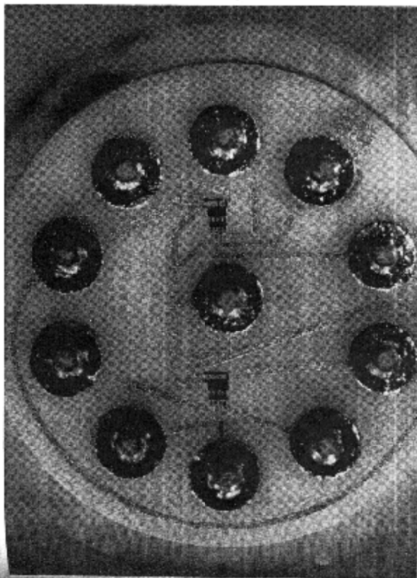
Fig. 10 — Two beam-lead integrated DCTL gates mounted on TO-5 header.
