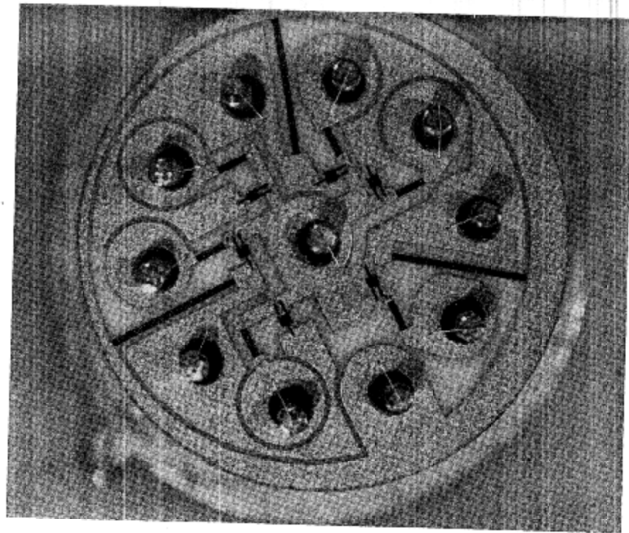
Fig. 7 — Hybrid thin-film digital circuit.
