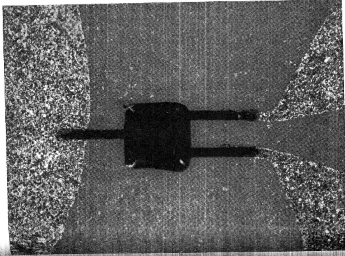
Fig. 2—Bonded beam-lead transistor.
