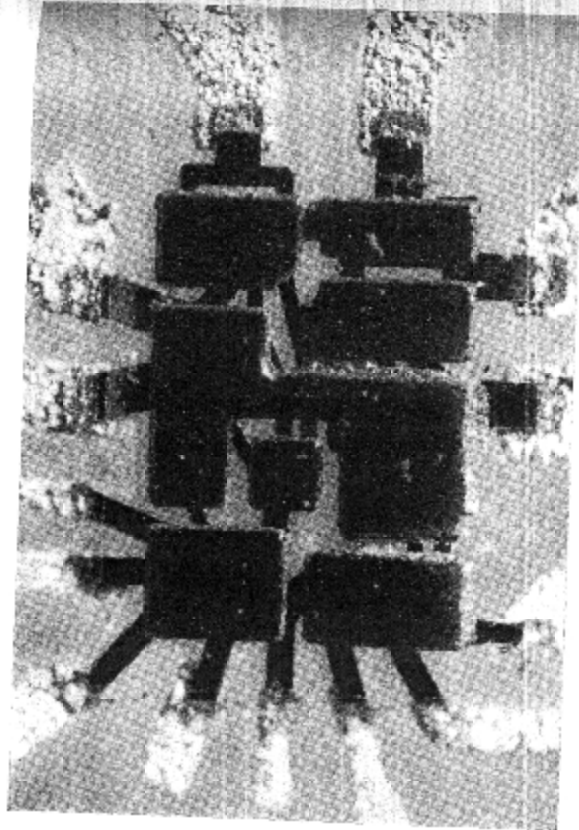
Fig. 11—Dual 4-input DTL gate mounted on gold-metallized substrate, 0.030 inch over-all.
