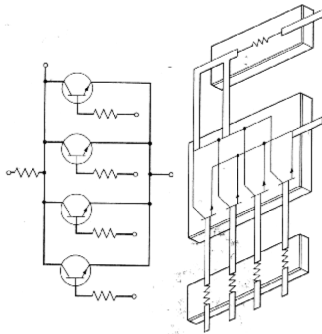
Fig. 8 — Circuit schematic of DCTL gate and physical-electrical schematic showing component placement.
