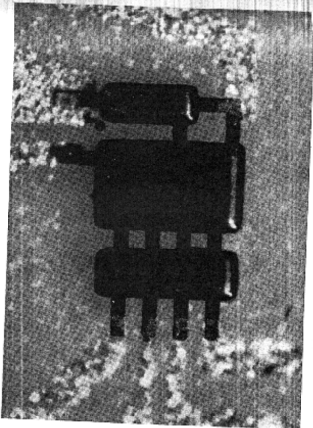
Fig. 9 — Beam-lead integrated DCTL gate mounted on gold-metallized ceramic, device side down.
