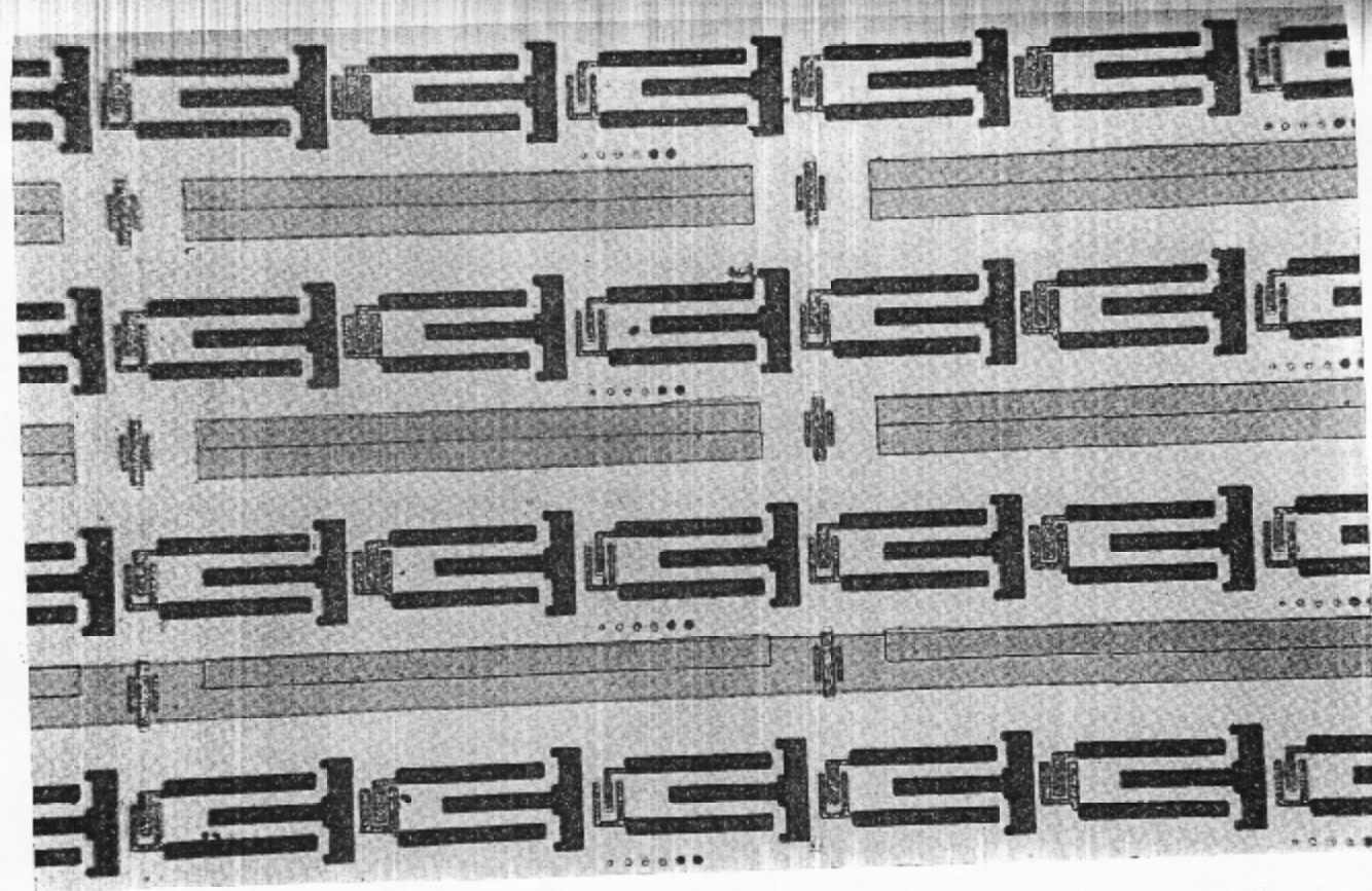
Fig. 3—Array of transistors.
